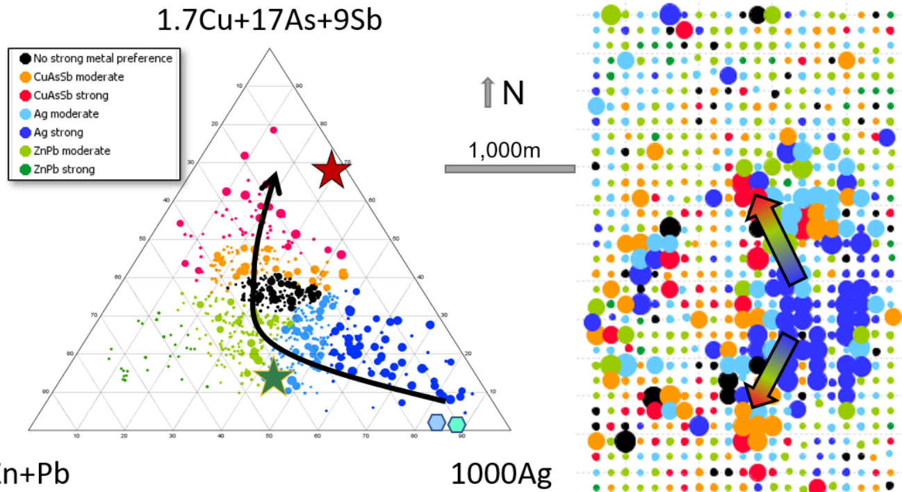
Figure 4 – Ternary plot showing the trend of mineralised zonation at the Mt Carlton HS system; The stars represent the gold rich ores and the hexagons the silver rich ores at Mt Carlton. The dots are the Fish Creek data. (LHS). This is represented in plan view at Fish Creek with the same colour scheme and emphasis is placed on the gold grades (dot sizes). Two anomalies similar to A39 and V2 at Mt Carlton are evident (RHS).
